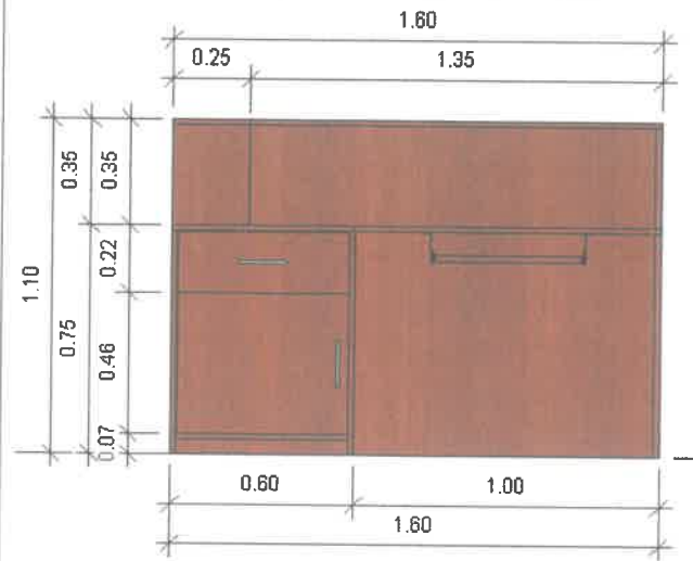
VISTA FRONTAL
