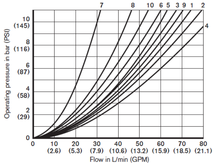
\Delta p - q_v -characteristic curves
